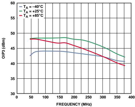
Figure 25. Output Third-Order Intercept vs. Frequency, Three Temperatures, Low Power Mode
