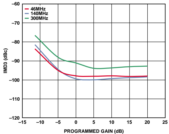
Figure 26. Two-Tone Output IMD3 vs. Programmed Gain at 46 MHz, 140 MHz, and 300 MHz; Low Power Mode
