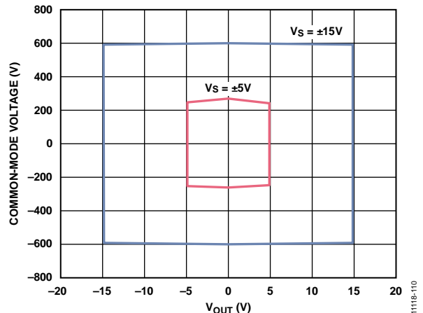
Figure 2. Input Common-Mode Voltage vs. Output Voltage
