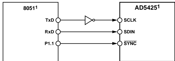
Figure 42. 80C51/80L51-to-AD5425 Interface
