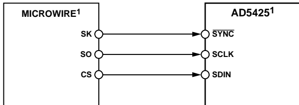
Figure 44. MICROWIRE-to-AD5425 Interface
