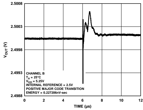
Figure 33. Digital-to-Analog Glitch Impulse
